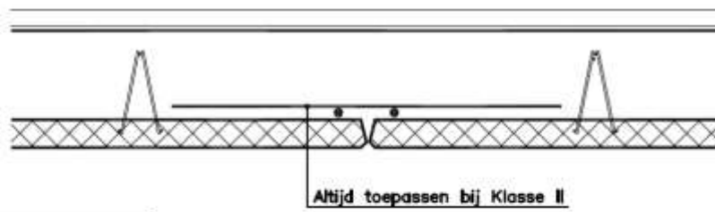
Detail VIII
