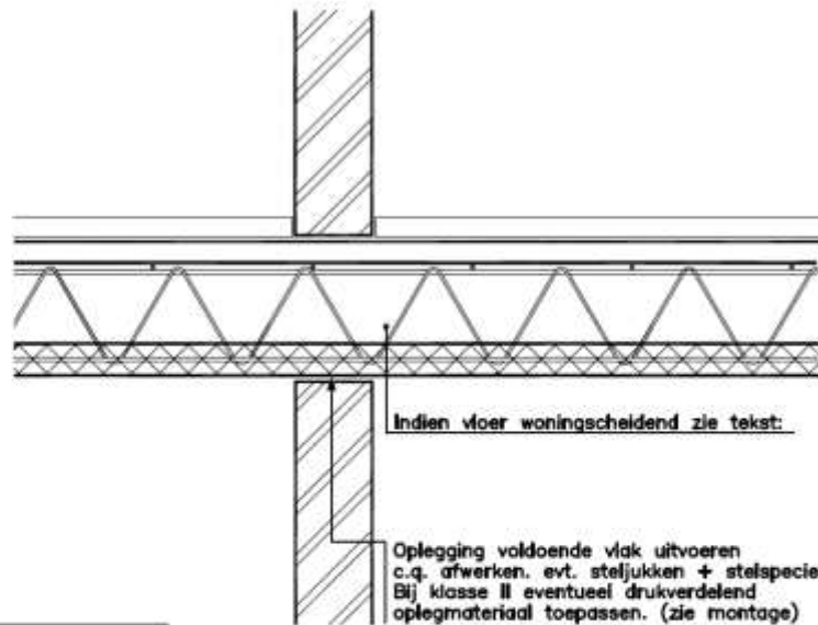
Detail III
